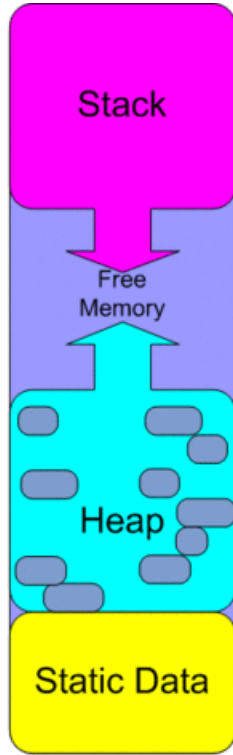
Fragmented Heap
