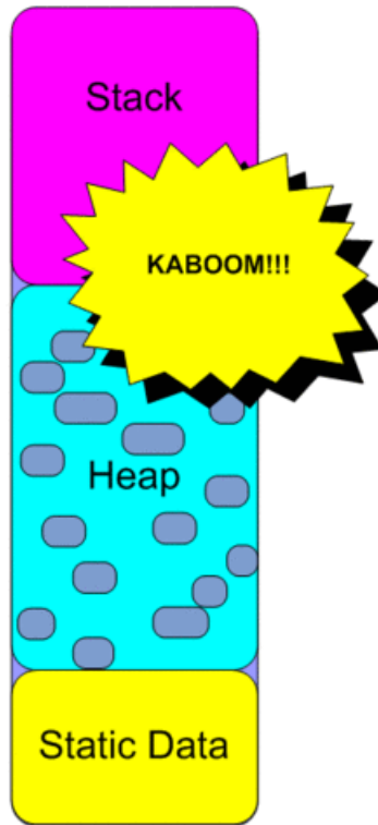
Stack Crash!
